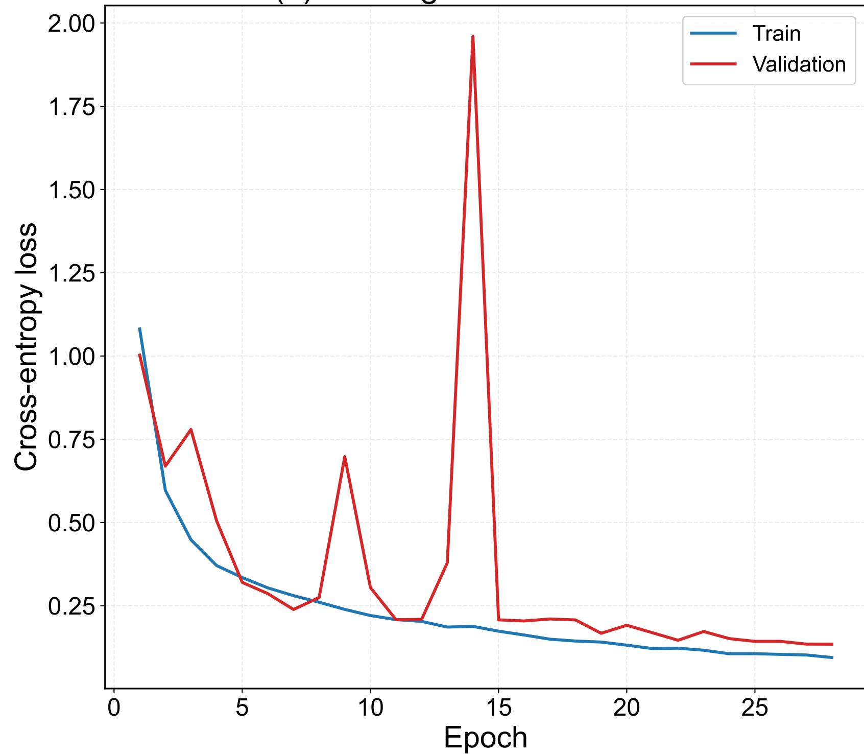
(b) Training & Validation Loss
