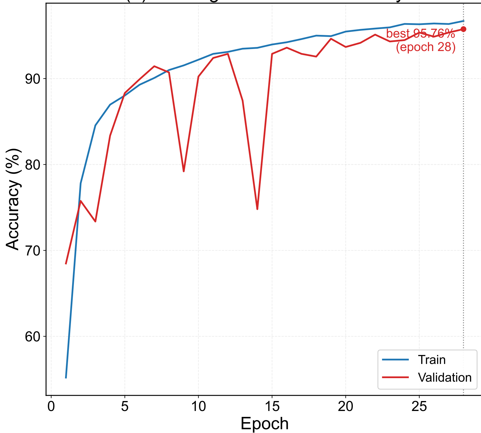
(a) Training & Validation Accuracy
